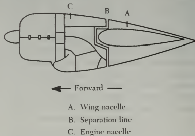
FIGURE 8-2. Typical engine and wing nacelle.
